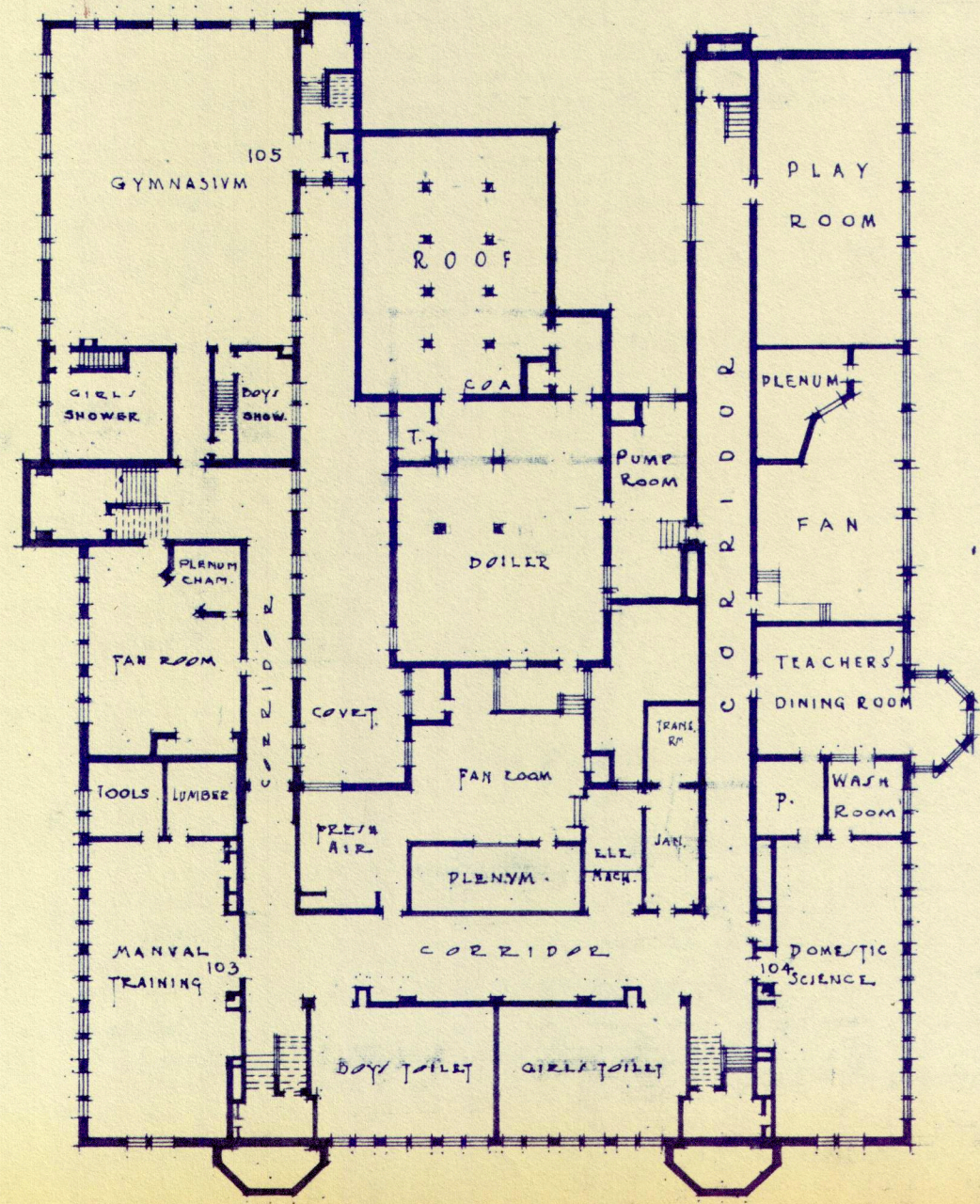
BASEMENT PLAN
