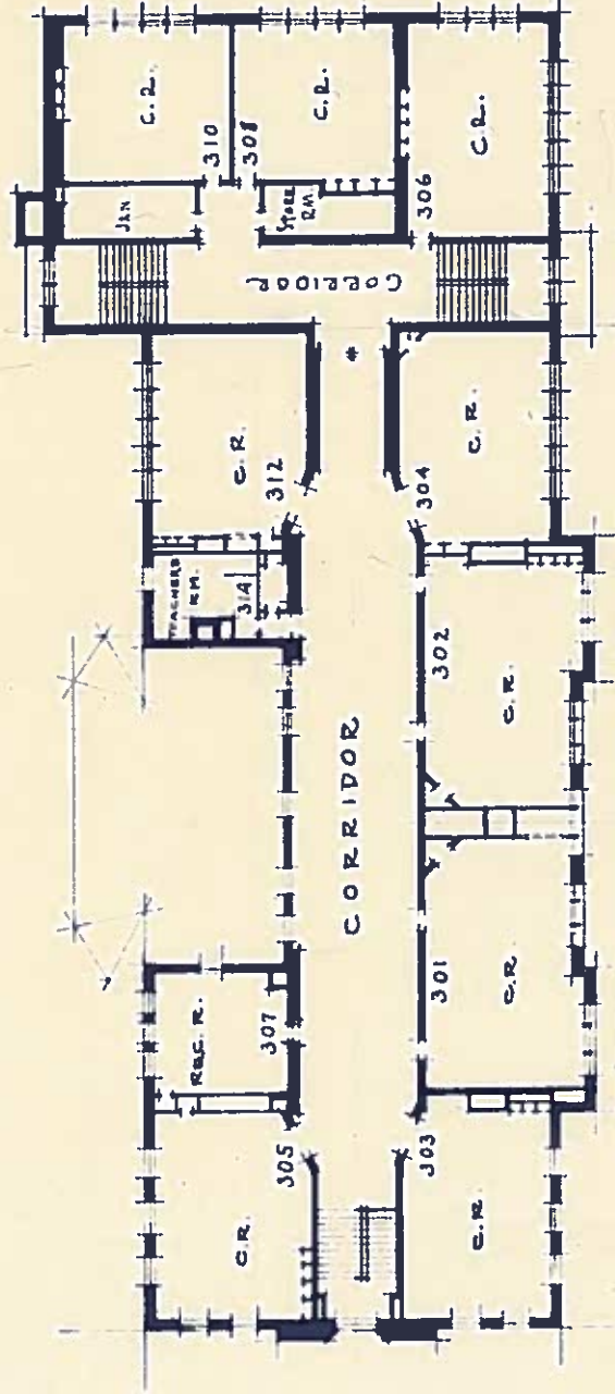
SECOND FLOOR PLAN Scale \frac{1}{32} = 1'-0"
