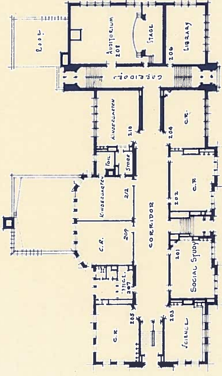
FIRST FLOOR PLAN SCALE \frac{3}{8}'' = 1'-0''
